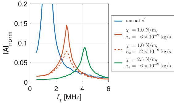
Fig. 5. Amplitude of oscillation normalized to that of the uncoated bubble ( R_0 = 2.5 \mu\text{m} ). The resonance curves shift toward higher frequencies with increasing shell stiffness \chi and broaden with increasing shell damping \kappa_s . The other parameters are as follows: driving pressure P_A = 1 \text{ kPa} ; ambient pressure P_0 = 100 \text{ kPa} ; surface tension of water \sigma = 72 \text{ mN/m} ; polytropic exponent \kappa = 1.07 ; liquid density \rho_L = 1000 \text{ kg/m}^3 ; speed of sound in the liquid c_L = 1500 \text{ m/s} ; liquid viscosity \mu_L = 2 \text{ mPa s} (to also account for thermal damping); and \sigma(R_0) = 20 \text{ mN/m} .
