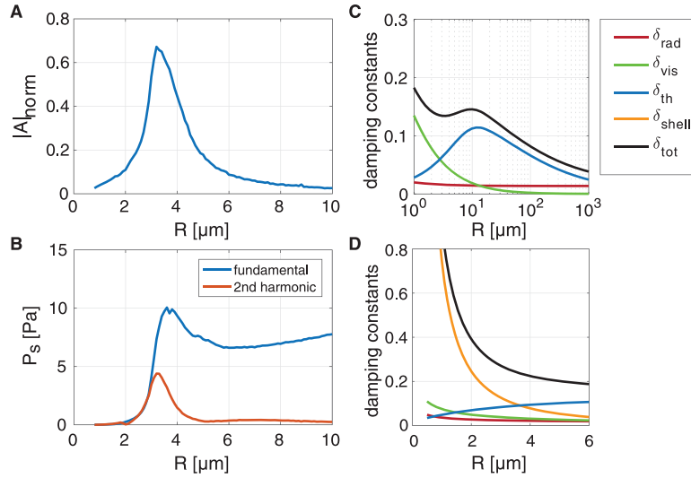
Fig. 4. (a) Maximum bubble response, expressed as the normalized amplitude ( i.e. , difference of maximum and minimum bubble amplitudes normalized by 2R_0 ) as a function of the bubble radius for a driving frequency of 1.0 MHz and a driving pressure of 75 kPa. Other parameters the same as in Figure 3. (b) The fundamental and second harmonic components of the scattered response of the bubble driven in (a) at a distance r = 2.54 cm. (c) The total damping \delta_{\text{tot}} of an uncoated bubble in water as a function of bubble size with damping contributions from sound reradiation \delta_{\text{rad}} , viscous damping \delta_{\text{vis}} owing to liquid viscosity and thermal damping \delta_{\text{th}} . (d) The total damping of a coated bubble ( \chi = 0.5 N/m) over the size range relevant for ultrasound contrast agents. The shell damping \delta_{\text{shell}} was calculated using a fixed shell viscosity \kappa_s = 1.0 \times 10^{-8} kg/s. Note that the total damping of a coated bubble is dominated by shell damping for bubbles in the diameter range 2–3 \mu\text{m} .
