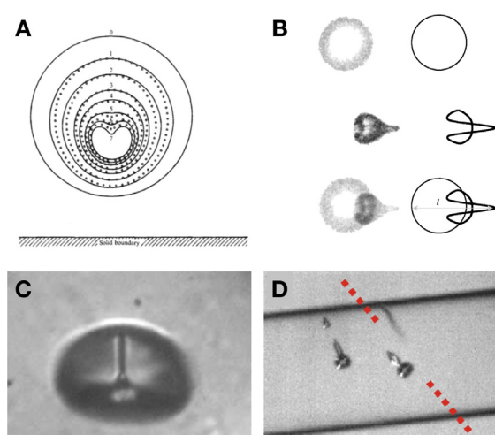
Fig. 9. Bubble jetting. (a) Calculated shape of a jetting bubble (reproduced with permission from Lauterborn and Bolle 1975); (b) jetting observed for a microbubble and a schematic representation of jet formation (reproduced with permission from Postema et al. 2005b); (c) jetting observed for a 3.0 \mu\text{m} lipid-coated bubble (reproduced with permission from Lajoinie et al. 2018); (d) SonoVue ultrasound contrast microbubbles driven at 200 kHz jetting in a capillary, with ultrasound beam (red dashed line; reproduced with permission from Cleve et al. 2019).
