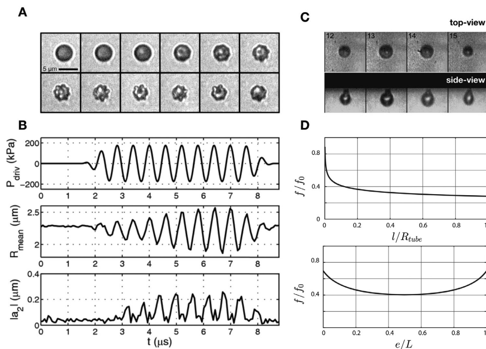
Fig. 8. (a) Evolution of the buildup of surface mode vibrations for echogenic liposomes. Asymmetric patterns indicative of surface mode oscillations are first visible, after several cycles of acoustic excitation (copyright Institute of Physics and Engineering in Medicine. Reproduced by permission of IOP Publishing from Raymond et al. 2016. All rights reserved). (b) Surface mode vibrations for BR-14 (Bracco Research) contrast agent. (Top) Applied acoustic pressure; (middle) radius-time curve; (bottom) evolution of mode 2, which saturates after about 4 cycles. Note the period-doubling behavior of the surface mode vibration (reproduced with permission from Dollet et al. 2008). (c) Top-view and side-view ultrahigh-speed imaging of ultrasound-driven contrast microbubbles (reproduced with permission from Vos et al. 2011). (d) Shift in the resonance frequency of a cylindrical bubble of length l as a function of initial length l_0 and axial location e within an open-ended tube of length L and radius R_{\text{tube}} (adapted from Oguz and Prosperetti 1998). In the top panel, L/R_{\text{tube}} = 10 and e/L = 0.5 ; in the bottom panel, L/R_{\text{tube}} = 10 and e/L = 0.17 .
