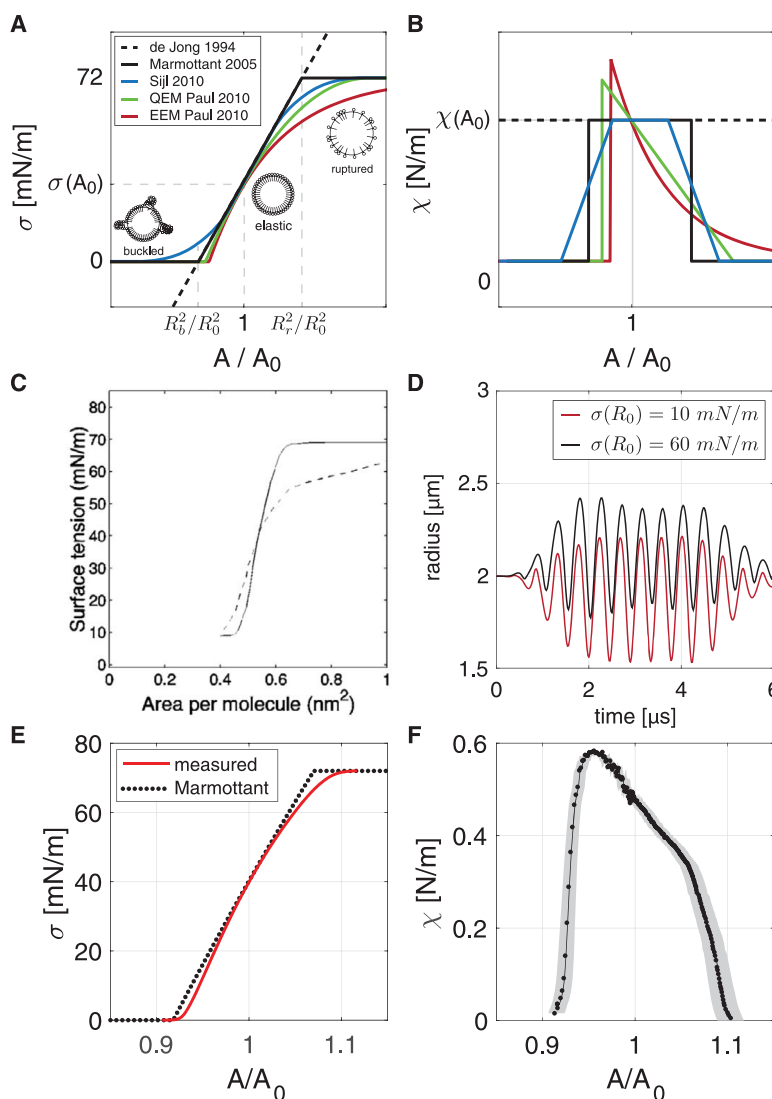
Fig. 6. (a) Ad hoc surface-tension curves implemented in Rayleigh–Plesset–type equations to account for shell elasticity (reproduced from Segers et al. 2018a by permission of The Royal Society of Chemistry); (b) shell stiffness ( \chi = A d\sigma / dA ) curves corresponding to the surface-tension curves plotted in (a) (reproduced from Segers et al. 2018a by permission of The Royal Society of Chemistry); (c) surface tension as a function of area per lipid molecule measured at slow dilatational rates in a Langmuir trough for disaturated phosphatidylcholine (DSPC) (solid line) and dipalmitoylphosphatidylglycerol (DPPG) (dotted line; reproduced with permission from Marmottant et al. 2005); (d) “compression-only” (red curve) and “expansion-only” (black curve) behavior modeled by limiting the surface tension between zero and that of the surrounding medium (solid curves in a); (e) measured surface-tension curve compared with Marmottant’s ad hoc implementation (reproduced from Segers et al. 2018a by permission of The Royal Society of Chemistry); (f) measured non-linear dilatational elasticity as a function of surface area (reproduced from Segers et al. 2018a by permission of The Royal Society of Chemistry).
