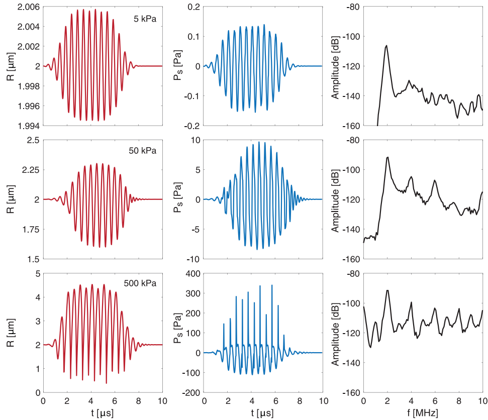
Fig. 3. (Left) Radius-time R(t) curves of a bubble with a radius R_0 = 2.0 \mu\text{m} at three different driving pressures: P_A = 5, 50 and 500 \text{ kPa} . The parameters for this system are as follows: ambient pressure P_0 = 100 \text{ kPa} ; surface tension \sigma = 72 \text{ mN/m} ; polytropic exponent \kappa = 1.07 ; speed of sound c_L = 1500 \text{ m/s} ; liquid density \rho_L = 1000 \text{ kg/m}^3 ; liquid viscosity \mu_L = 2.0 \text{ mPa s} (to account for thermal damping); shell elasticity \chi = 1.0 \text{ N/m} ; shell viscosity \kappa_s = 1.0 \times 10^{-8} \text{ kg/s} ; and initial surface tension \sigma(R_0) = 20 \text{ mN/m} . Ultrasound consisted of a Gaussian-tapered narrowband driving pulse with 16 cycles at a driving frequency of 2.0 \text{ MHz} . (Middle) Scattered pressure P_s(t) at a distance of r = 2.54 \text{ cm} at the three driving pressures. (Right) Spectral content of the scattered pressures.
