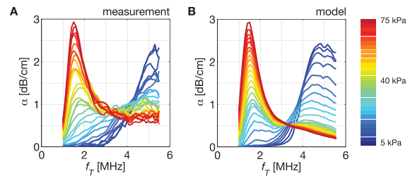
Fig. 7. (a) Attenuation of a monodisperse bubble sample (monodispersity achieved by acoustic sorting) measured at pressures ranging from 5 to 75 kPa (Segers and Versluis 2014); (b) modeled attenuation (reproduced with permission from Segers et al. 2016a).
