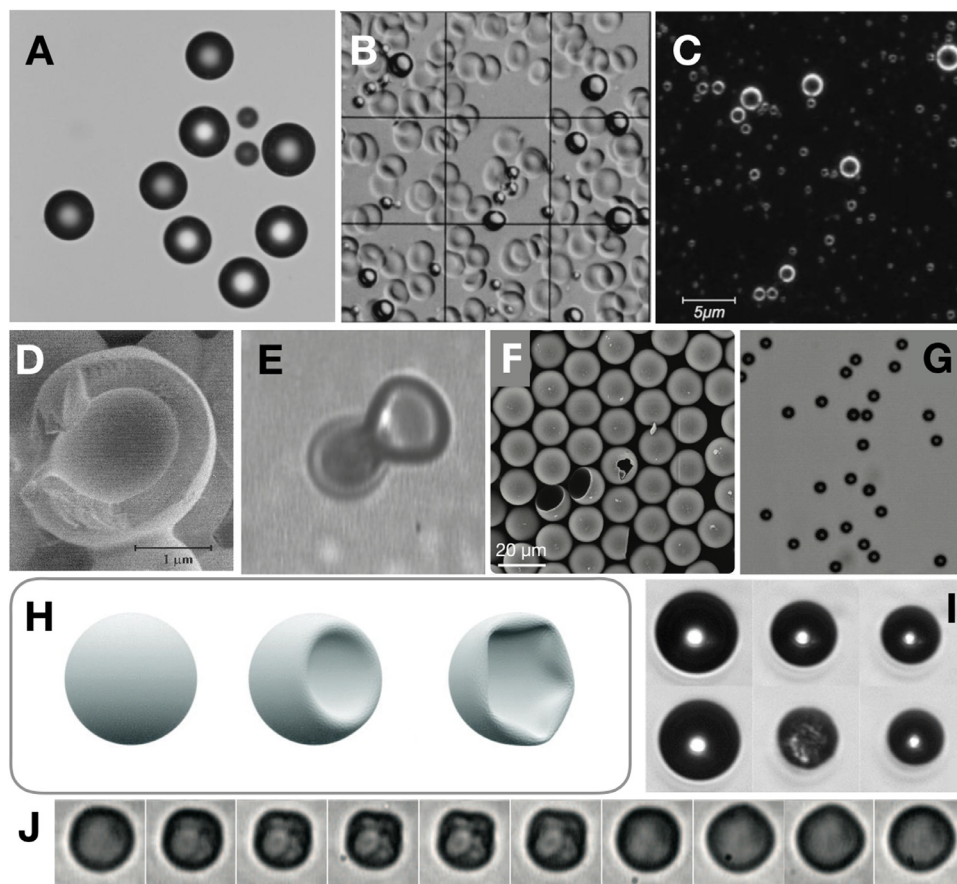
Fig. 1. Ultrasound contrast-agent microbubbles. (a) Lipid-coated microbubbles as seen in bright-field microscopy (reprinted with permission from Segers et al. 2016b. Copyright 2016 American Chemical Society); (b) perfluoropropane bubbles with a protein shell (Optison), seen here against a background of red blood cells (reproduced from Wilson and Burns 2010); (c) lipid-coated microbubbles of perfluoropropane gas (Definity) as seen in dark-field microscopy (reproduced from Wilson and Burns 2010); (d) scanning electron micrograph of a Quantison microsphere, fractured owing to vacuum (reproduced with permission from Frinking and de Jong 1998); (e) vapor bubble release from a laser-heated single oil-filled microcapsule captured under ultrahigh-speed imaging (reproduced with permission from Lajoinie et al. 2014); (f) scanning electron micrograph of monodisperse microcapsules (image courtesy of Nanomi, Oldenzaal, the Netherlands); (g) monodisperse microbubbles with a radius of 2.7\ \mu\text{m} produced in a flow-focusing device (reprinted with permission from Segers et al. 2016b. Copyright 2016 American Chemical Society); (h) numerical simulation of the buckling instability of the elastic shell of a polymeric hard-shelled microcapsule (reproduced with permission from Marmottant et al. 2011); (i) buckling instability upon dissolution for two different surfactants (Survanta and dipalmitoylphosphatidylcholine (DPPC)) (reprinted with permission from Thomas and Borden 2017. Copyright 2017 American Chemical Society); (j) buckling observed during compression of a lipid-coated microbubble (reproduced with permission from Sijl et al. 2011).
