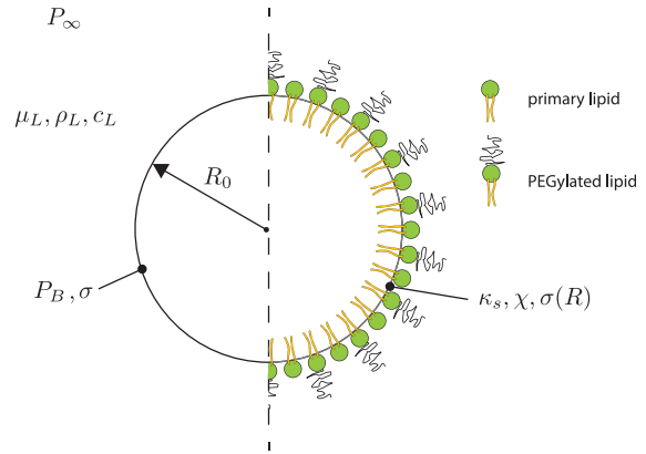
Fig. 2. Schematic view of a free gas bubble ( left ) and a lipid-coated microbubble ( right ). To the right, the coating is indicated by the primary phospholipids and lipids with polyethylene glycol added (not drawn to scale). R_0 = bubble size; P_B = liquid pressure at the bubble wall; P_\infty = liquid pressure far away from the bubble; \mu_L = liquid viscosity; \rho_L = liquid density; c_L = speed of sound in the liquid; \sigma = surface tension of water; \kappa_s = shell viscosity; \chi = shell elasticity; \sigma(R) = size-dependent effective surface tension of the coated bubble.
