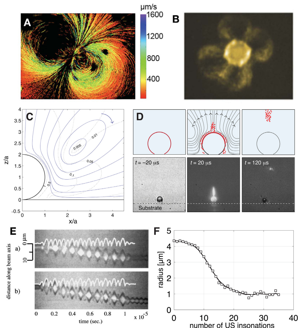
Fig. 10. (a) Microstreaming field as a result of an oscillating SonoVue microbubble (reproduced with permission from Pereno et al. 2018 ). (b) Lipid shedding and transport as a result of acoustic streaming (reproduced with permission from Versluis 2013 ). (c) Simulation of the acoustic streaming generated by an oscillating bubble of radius a (the half-circle) in contact with a plane wall located at z=0 . Only half of the space is sketched, owing to axisymmetry about the x=0 axis. The solid curves are the streamlines, and the direction of velocity is indicated with the arrows; in particular, the streaming flow goes away from the wall above the bubble (reproduced with permission from Marmottant et al. 2006 ). (d) Lipid shedding from a targeted bubble and transport by acoustic streaming. (Top) Schematics of the shedding process of the released material (red) with the calculated streamlines (solid black lines); (bottom) experimental recording of the release of the fluorescent material from a targeted oscillating microbubble driven at a pressure of 331 kPa, showing transport over a distance several times larger than the bubble size (reproduced with permission from Lajoinie et al. 2018 ). (E) Streak imaging of two ultrasound contrast agents of equilibrium radius 2.1 \mu\text{m} (top) and 2.0 \mu\text{m} (bottom), showing the displacement in the direction of propagation of the acoustic wave. The acoustic forcing represents 20 cycles at amplitude 380 kPa and frequency 2.25 MHz. These snapshots are overlaid with simulated curves of the time evolution of the bubble radius (reproduced with permission from Dayton et al. 2002 ). (F) Evolution of the radius of a lipid-coated microbubble subjected to repeated acoustic pulses (frequency 2.25 MHz, peak negative pressure 400 kPa, pulse repetition frequency 0.5 Hz; data kindly provided by Mark Borden).
